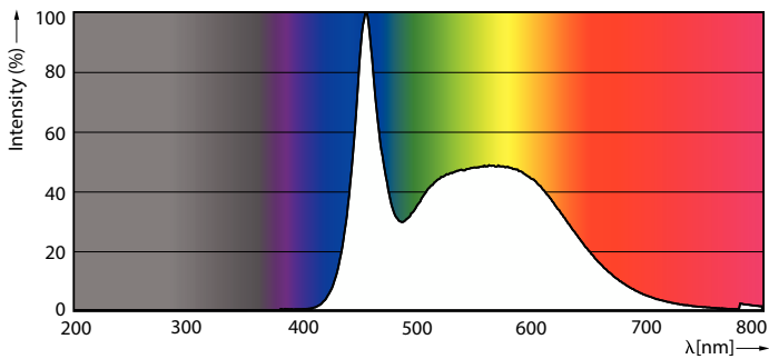
Spectral Power Distribution Colour - EcoHome LEDBulb 10W E27 6500KLV 1PF/20
