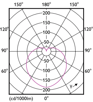
Light Distribution Diagram - EcoHome LEDBulb 10W E27 6500KLV 1PF/20
