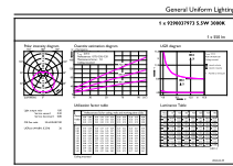
Light Distribution Diagram - EcoHome LEDBulb 5.5W E27 3000KLV 1PF/20
