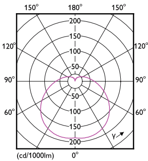
Light Distribution Diagram - EcoHome LEDBulb 5.5W E27 3000KLV 1PF/20
