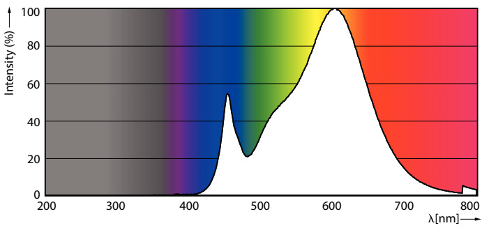
Spectral Power Distribution Colour - EcoHome LEDBulb 5.5W E27 3000KLV 1PF/20
