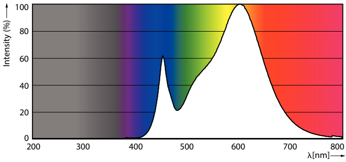
Spectral Power Distribution Colour - EcoHome LEDBulb 14W E27 3000KLV 1PF/20
