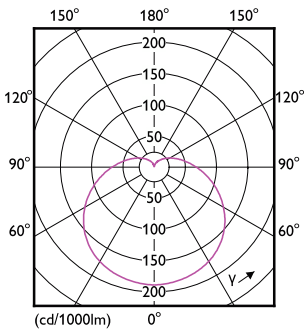
Light Distribution Diagram - EcoHome LEDBulb 14W E27 3000KLV 1PF/20
