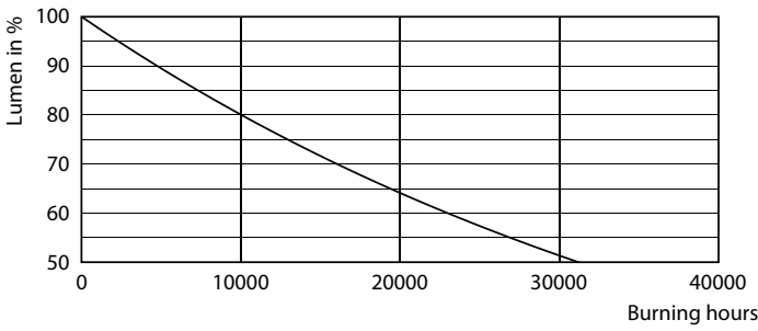
Lumen Maintenance Diagram - EcoHome LEDBulb 14W E27 3000KLV 1PF/20
